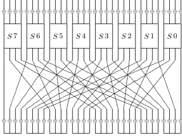
Fig. 4. One round of SMALLPRESENT-[8] and PRESENT/SMALLPRESENT S-box.
