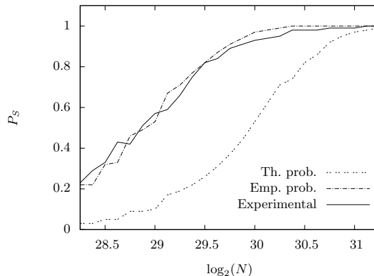
Fig. 2. Success probability of an attack on SMALLPRESENT-[8] with the 40-bit key-schedule
