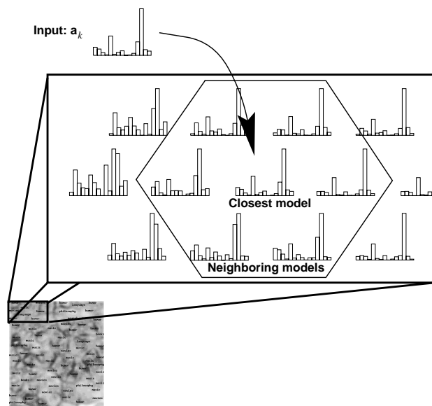
Figure 2: The Self-Organizing Map consists of a set of model vectors, depicted here as histograms where each bin corresponds to one component. The models are attached onto a map lattice at regularly spaced intervals. An example map display of a document collection is shown in the lower left corner, and the enlarged portion shows the map lattice that underlies the top left corner of the map display. The arrow illustrates the mapping of the document vector \mathbf{a}_k , and the hexagon denotes the neighborhood of the closest model.
