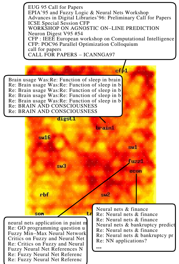
Figure 4: A map of neural network discussions organized with the WEBSOM method. The short, manually inserted labels, “bookmarks”, on the map describe the underlying map area (their explanations have been omitted here for brevity). The titles of the documents found in four sample map nodes are shown in the boxes.
