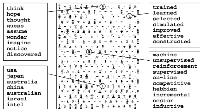
Figure 3: Sample word categories on a self-organized semantic map. Each inset shows the words that have been mapped into one word category. The text corpus consisted of articles from the Usenet newsgroup comp.ai.neural-nets .
