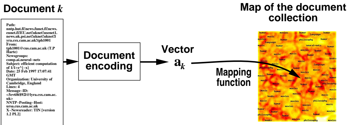
Figure 1: The basic building blocks of the WEBSOM system.
