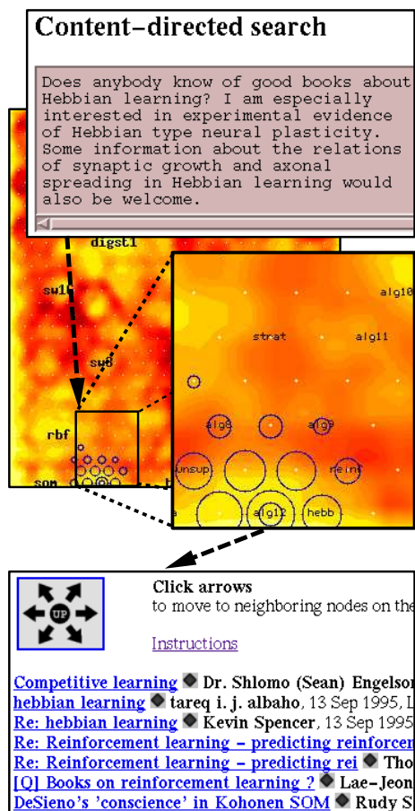
Figure 6: A new document or any written description can be used for finding related documents. The circles on the map display denote the locations that best represent the textual description shown in the topmost display. Titles of some of the articles found in the best matching map location are shown in the display at the bottom.
