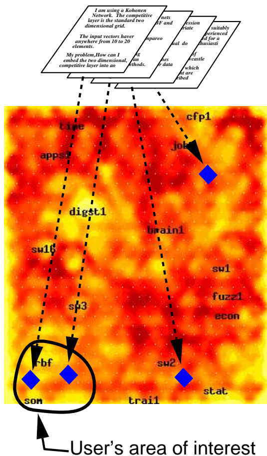
Figure 7: The document map can be used as a filter that notifies the user of interesting documents. Any interesting area on the map can be marked as a trap which keeps the new documents.
