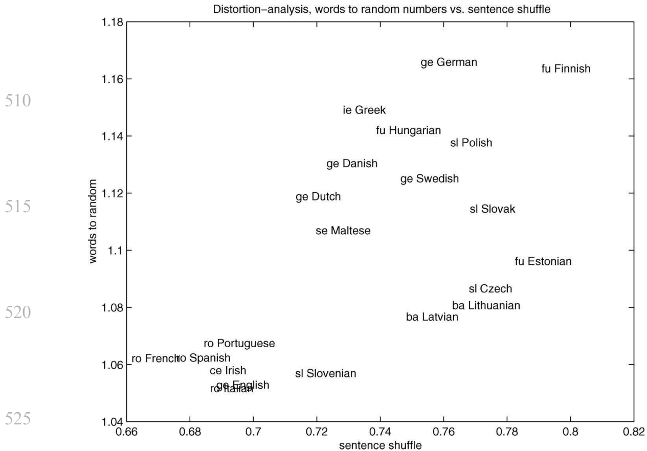
Fig. 4. Language map: morphology vs. word order information.
