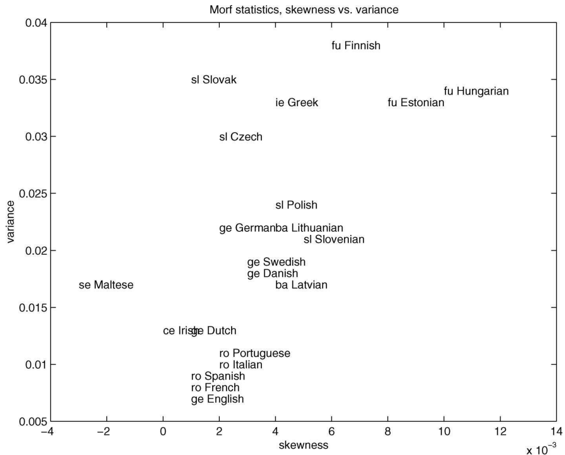
Fig. 10. Average “skewness” and “variance” of morph lengths.
