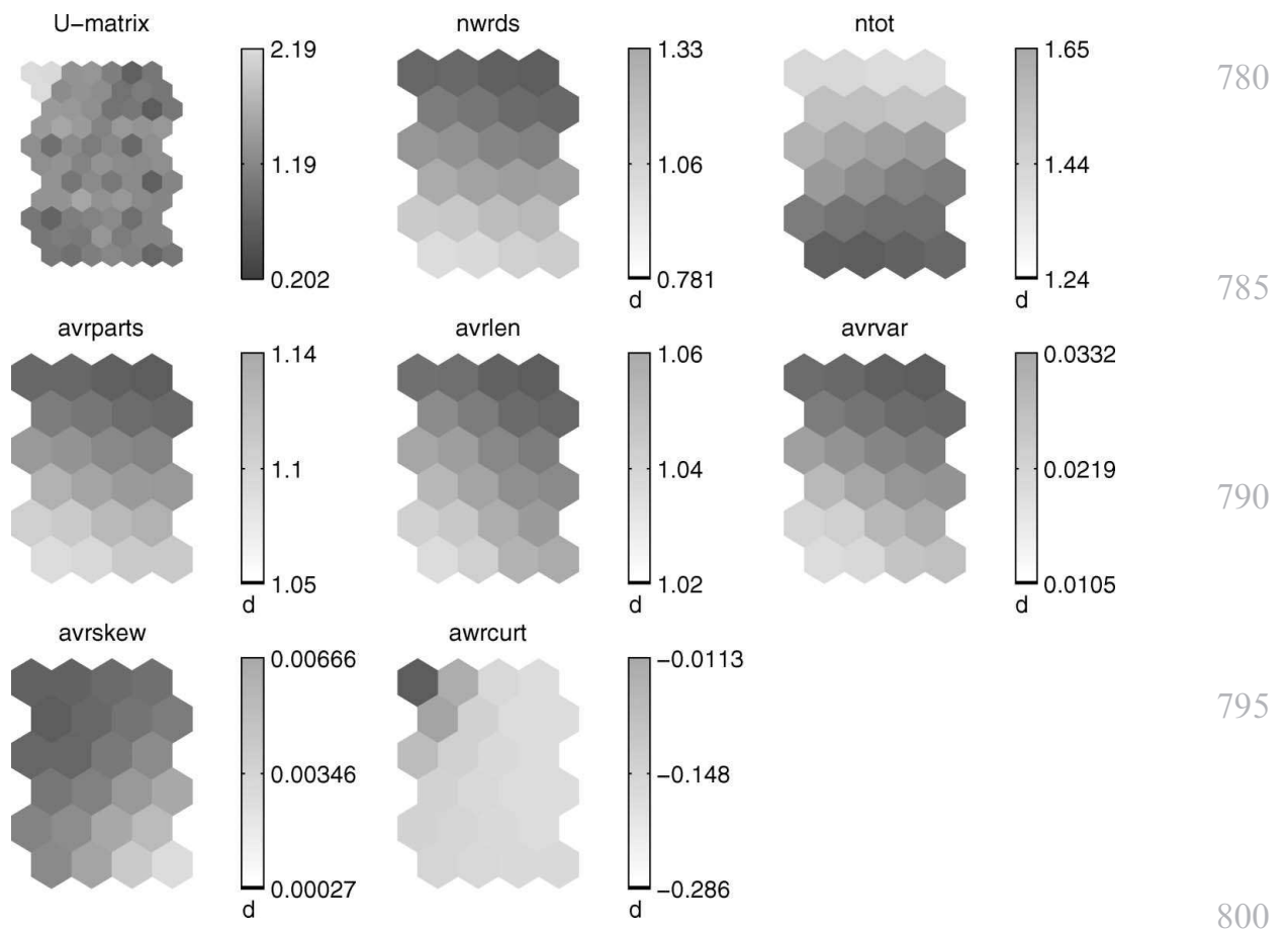
Fig. 8. The distribution of the variables on the map; see text for the explanation of the variables.
