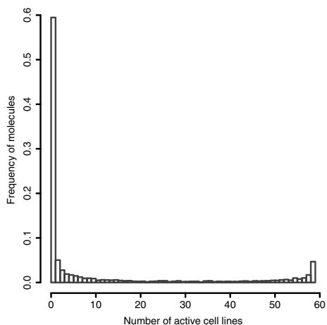
Fig. 1. Skewness of the multilabel distribution
