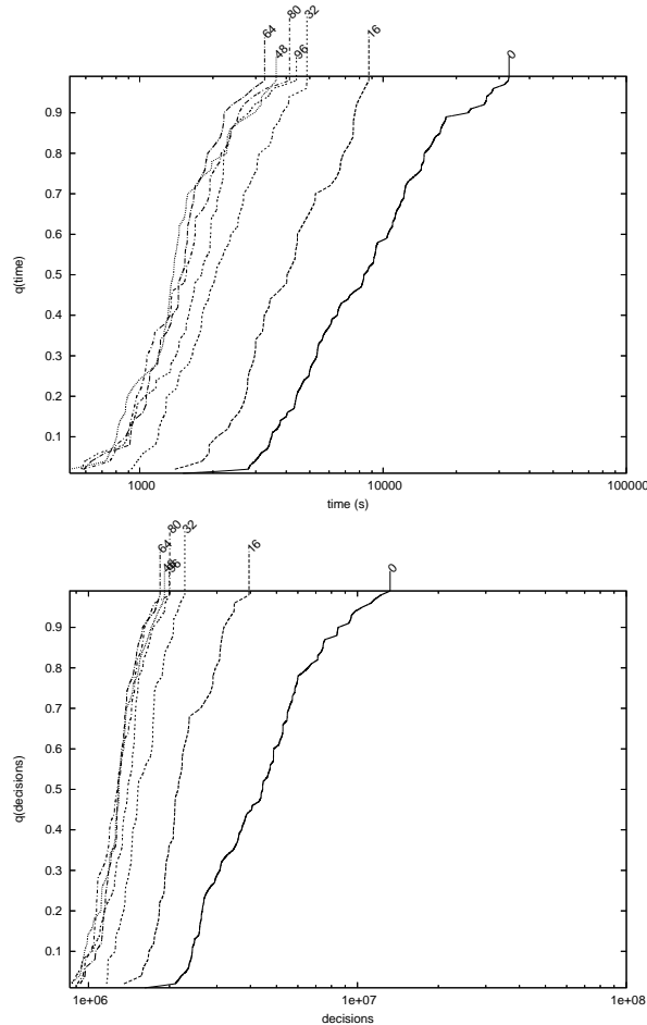
Figure 6.4: Distributions for run time and number of decisions for mano1 using different values of preceding jobs r and ChooseLen
