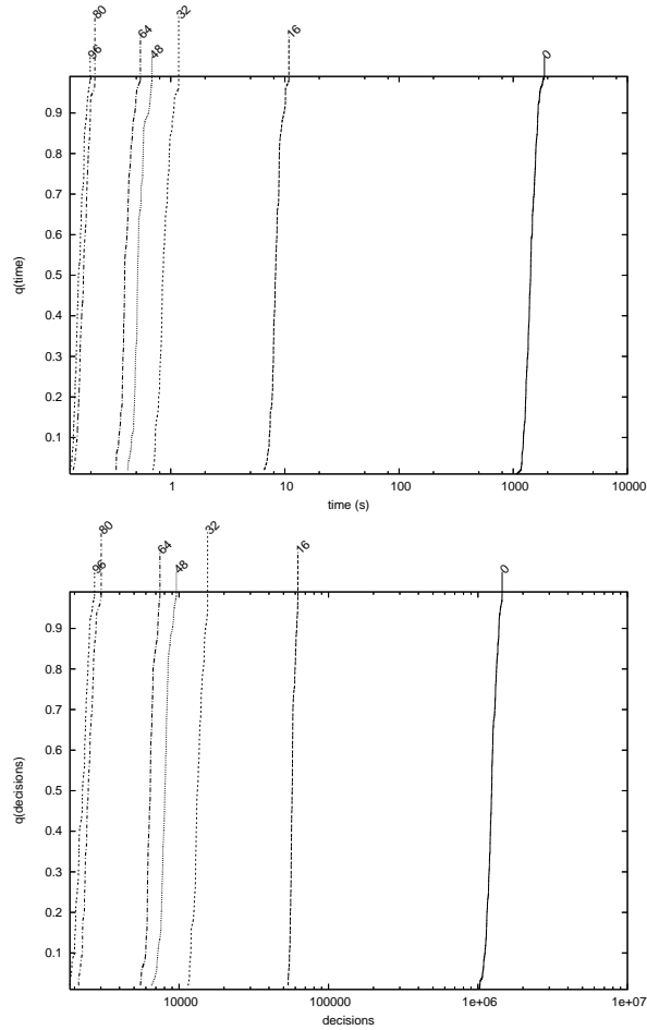
Figure 6.3: Distributions for run time and number of decisions for contest using different values of preceding jobs r and ChooseLen
